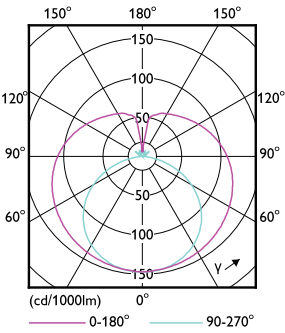
Light Distribution Diagram - Ledtube DE 1200mm 19W 865 T8 G13 EG
